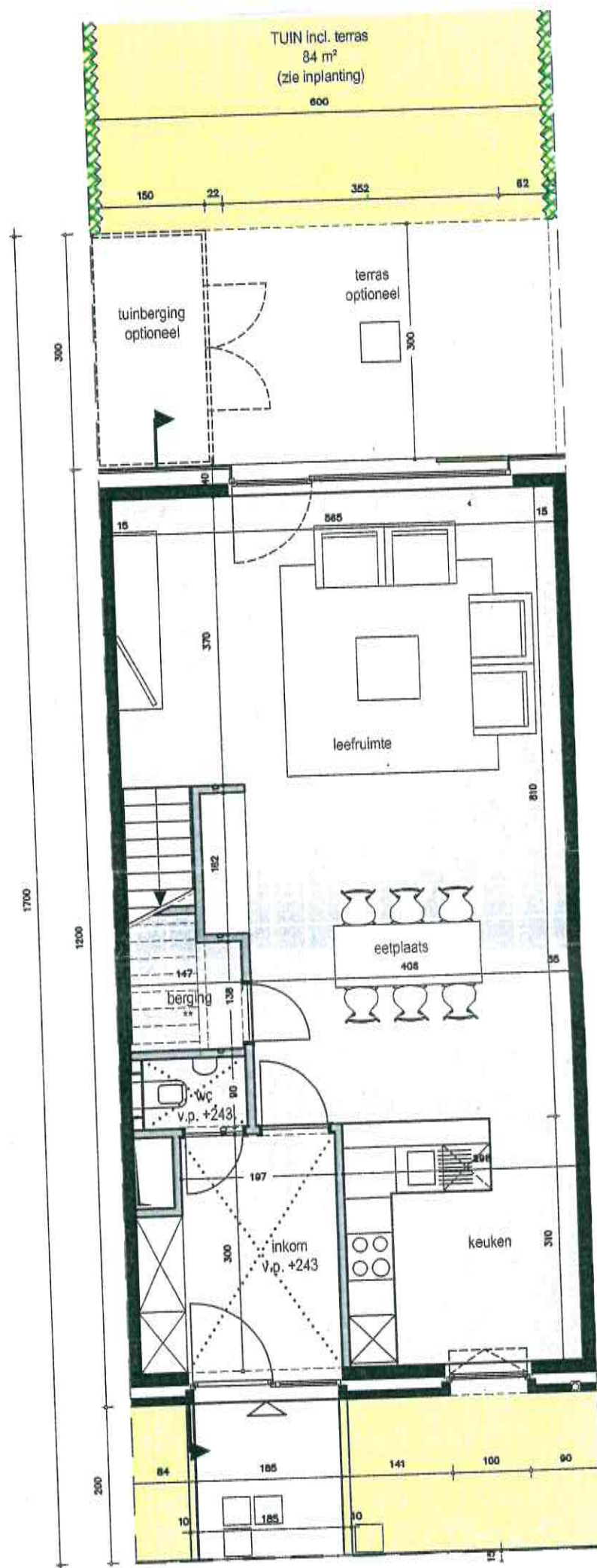
plan 00 schaal 1/100
